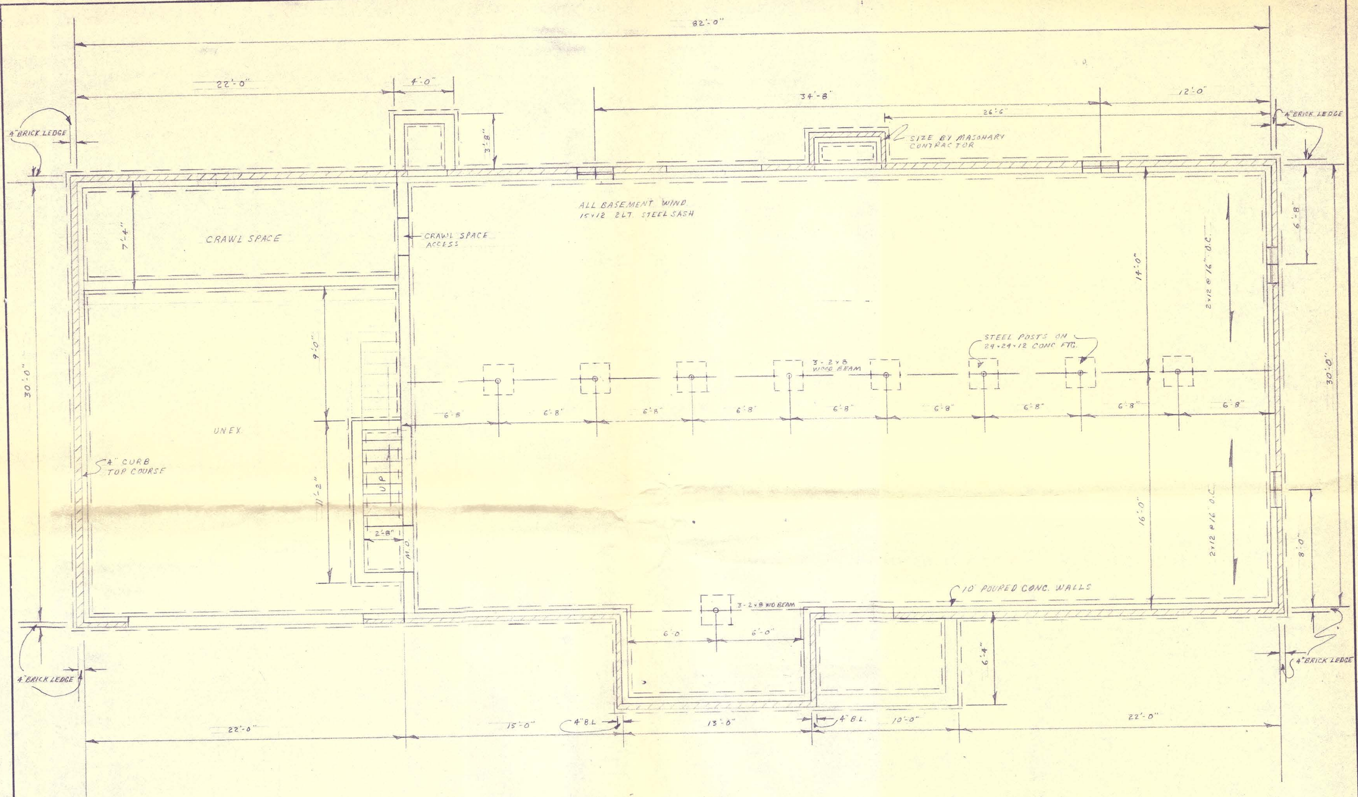
BASEMENT & FOUNDATION PLAN SCALE 1/4" = 1'-0"
